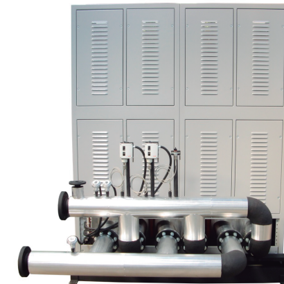
DIFHEMI – ALCOA Italy, 990KW for Thermal Fluid at 300 °C, pressure 6 Bar
