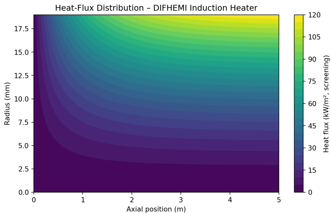
Figure 5. CFD_heatflux_induction
