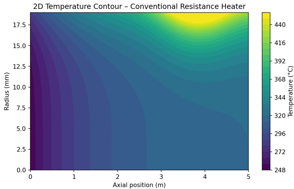
Figure 4. CFD_2D_Resistance_units
