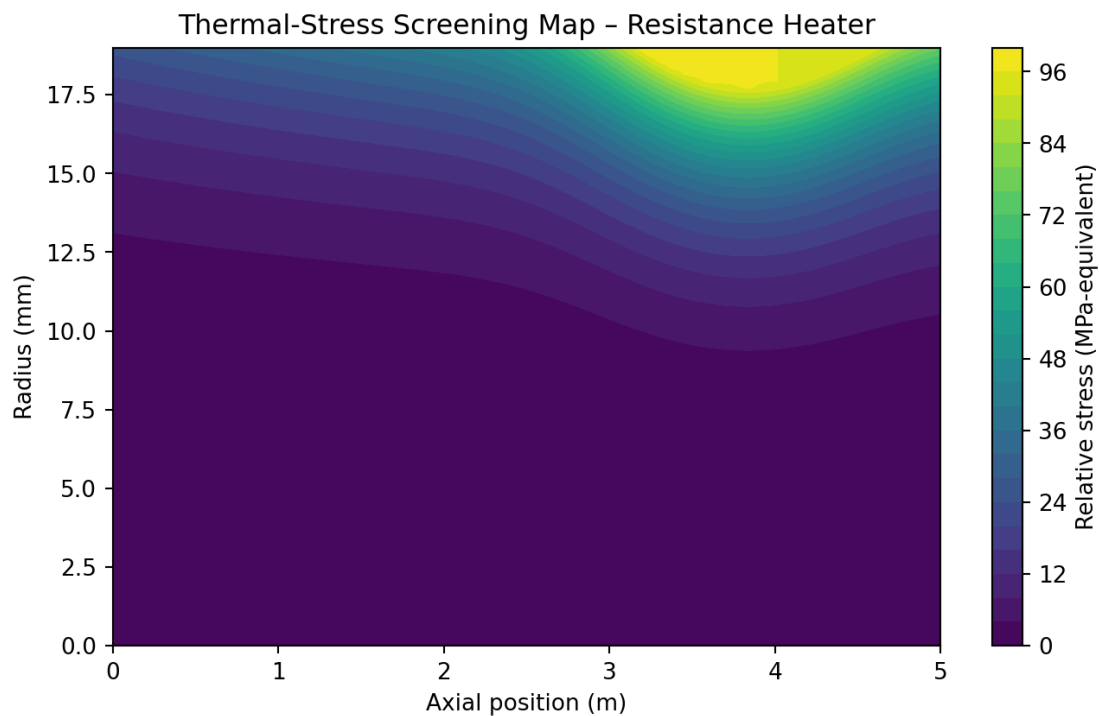
Figure 8. CFD_stress_resistance
