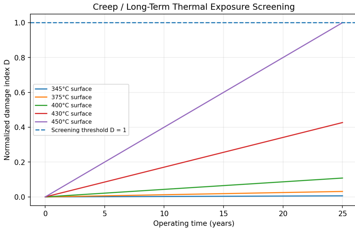
Figure 9. creep_life_damage_index
