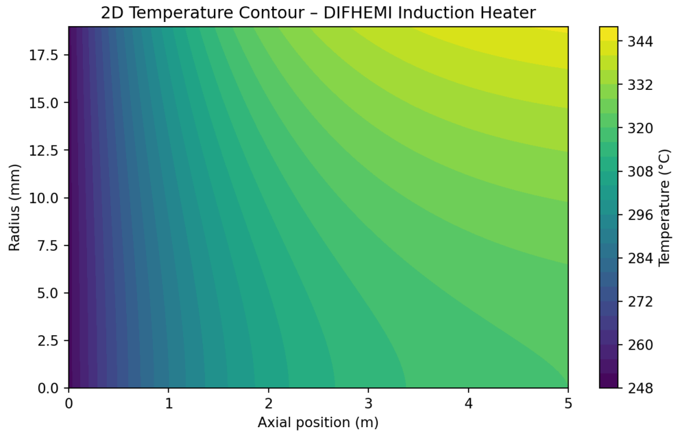
Figure 3. CFD_2D_Induction_units
