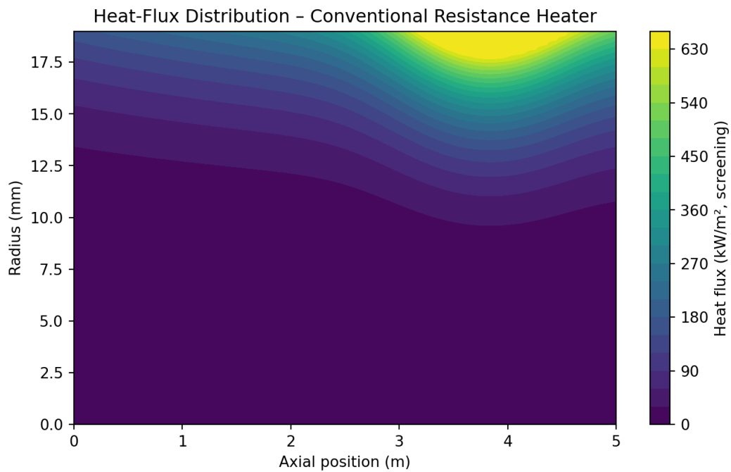
Figure 6. CFD_heatflux_resistance
