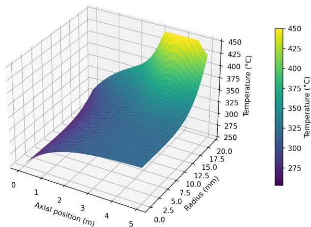
Figure 2. CFD_3D_Resistance_units
