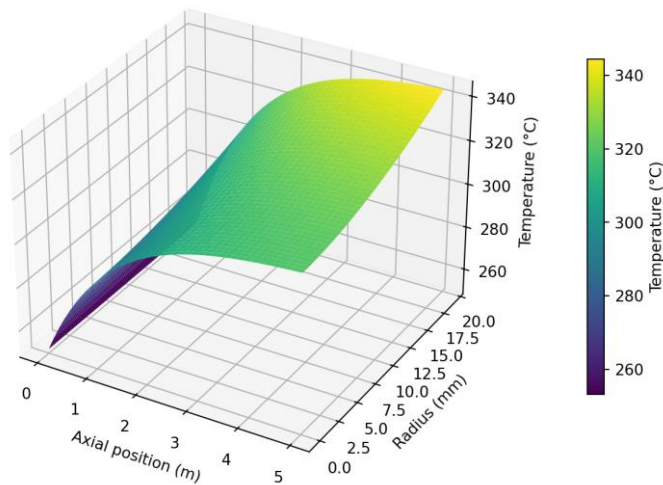
3D Temperature Field – DIFHEMI Induction Heater
