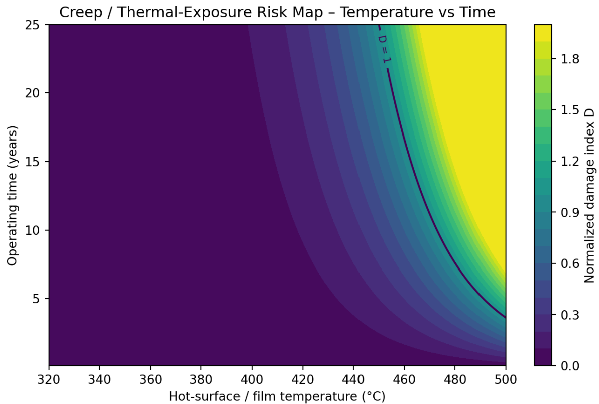
Figure 10. creep_risk_map_temperature_time
